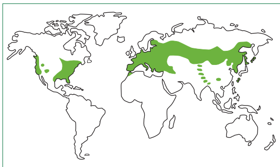
Figure 2: World-wide distribution of ixodid ticks capable of carrying and transmitting B burgdorferi to humans Reproduced with permission of WHO.
